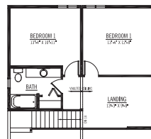
DORMER OPTION 2 LOFT PLAN 610 SQFT.
