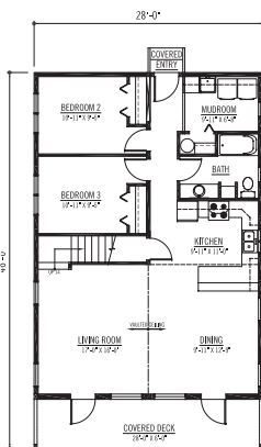
MAIN FLOOR PLAN 1120 SQFT.
