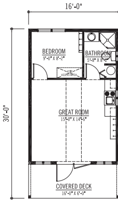
OPTION 1 MAIN FLOOR PLAN 384 SQFT.
