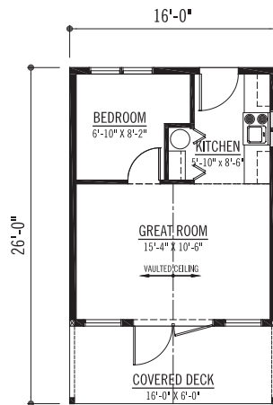
OPTION 2 FLOOR PLAN 320 SQFT.
