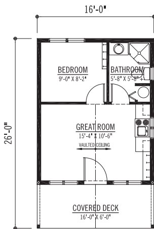
OPTION 1 FLOOR PLAN 320 SQFT.
