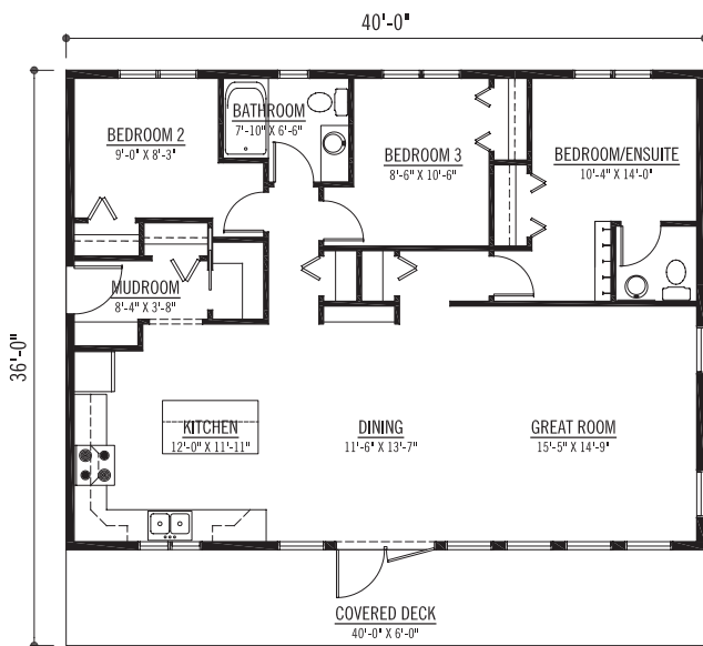
FLOOR PLAN 1200 SQFT.
