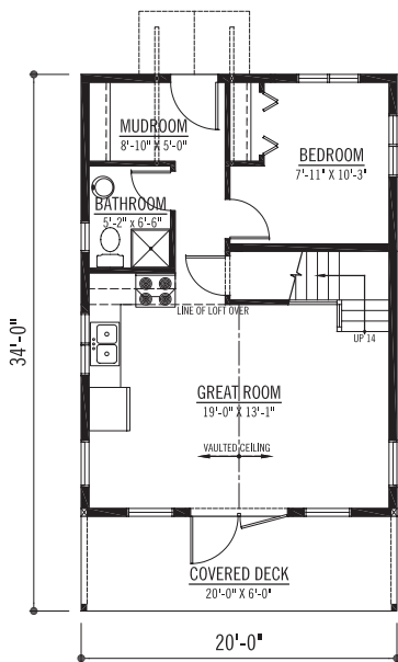
MAIN FLOOR PLAN
