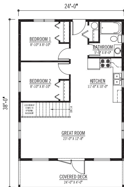
FLOOR PLAN 768 SQFT.
